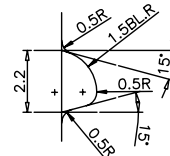
THREAD DETAIL SCALE 10:1
